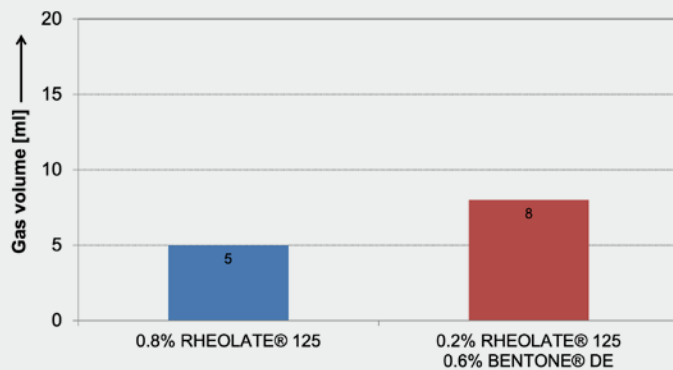
FIGURE 5: Gassing stability at 40°C
