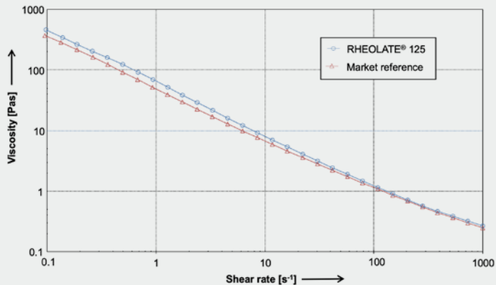
FIGURE 2: Flow characteristics
