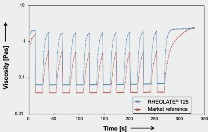
FIGURE 3: Circulation stability
