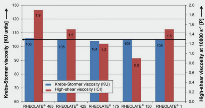
FIGURE 2: Comparison of high- and mid-shear viscosity
