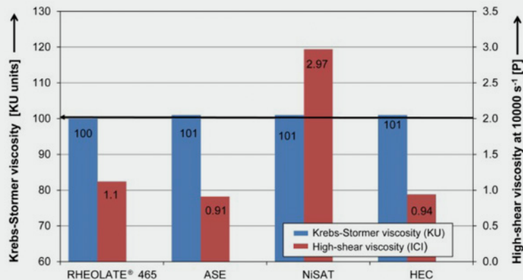
FIGURE 9: Comparison of high- and mid-shear viscosity
