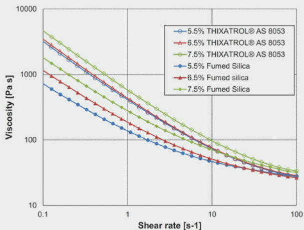
FIGURE 9: Rheology clear SPUR sealant
