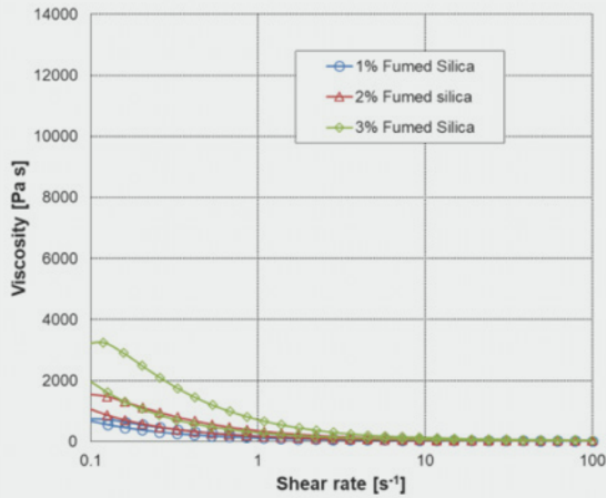
FIGURE 4B: Fumed silica in SPUR
