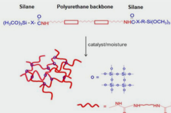
FIGURE 1: Curing mechanism of SPUR polymer
