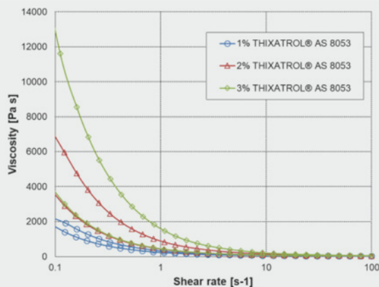
FIGURE 4A: THIXATROL® AS 8053 in SPUR
