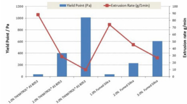
FIGURE 6: Yield value vs extrusion rate
